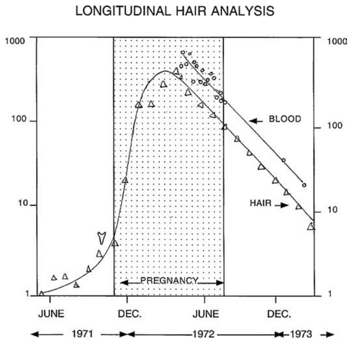
FIG. 11. The concentration of mercury in consecutive 1-cm segments of a maternal sample and corresponding concentration in blood samples. The dotted band is the period of pregnancy. The vertical arrow indicates the estimated date for the start of consumption of the contaminated bread.
